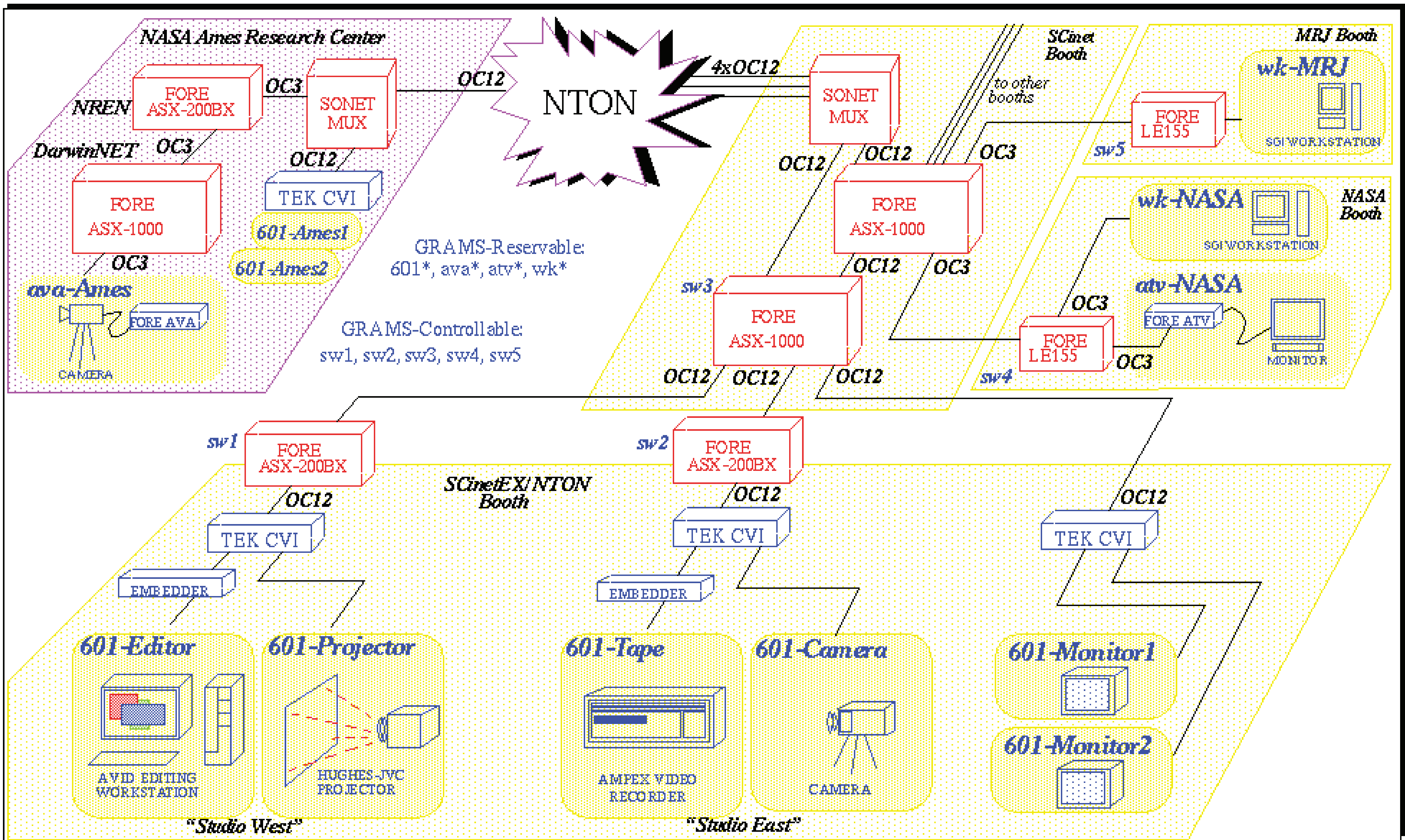
FIGURE 1. Experimental ATM Network
