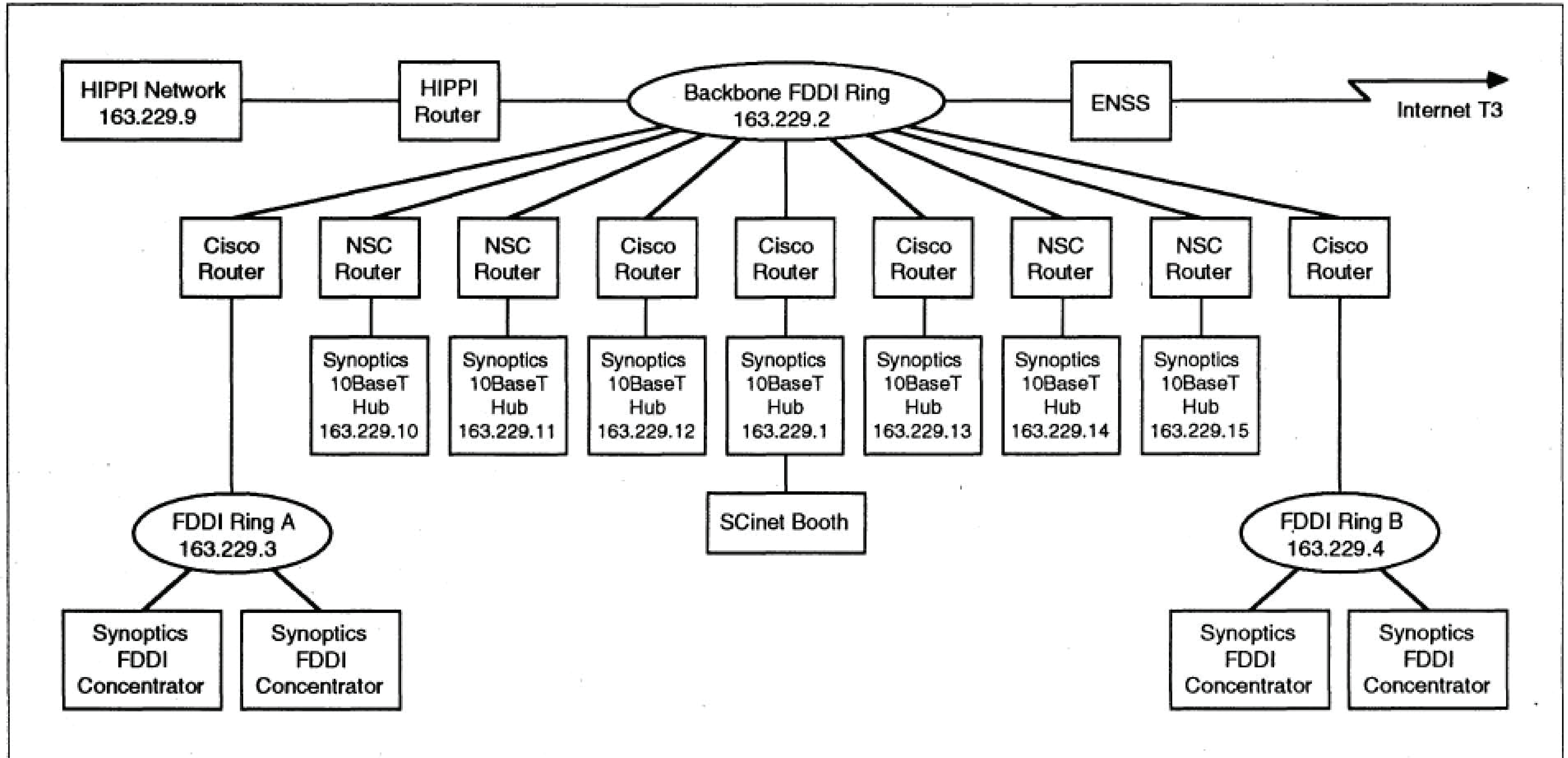
Figure 1. SCinet '92 network architecture
